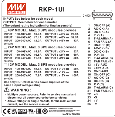
Figure 1-2: Safety labels of RKP-1U□
