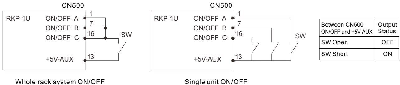
Figure 3-4 Connection for remote ON/OFF control operation
