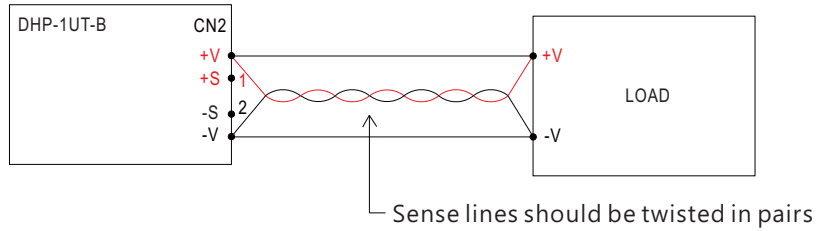
Figure 5-8 Connection of Remote Sense
