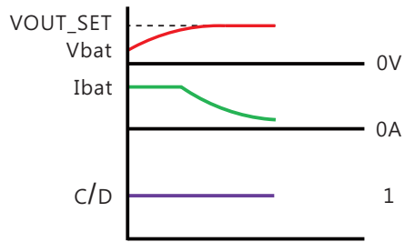
VOUT_SET higher than Vbat and C/D=1
