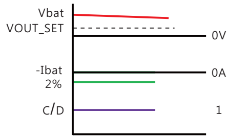
VOUT_SET lower than Vbat and C/D=1
