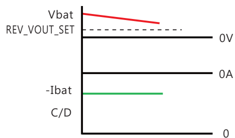
VOUT_SET_REV lower than Vbat and C/D=0
